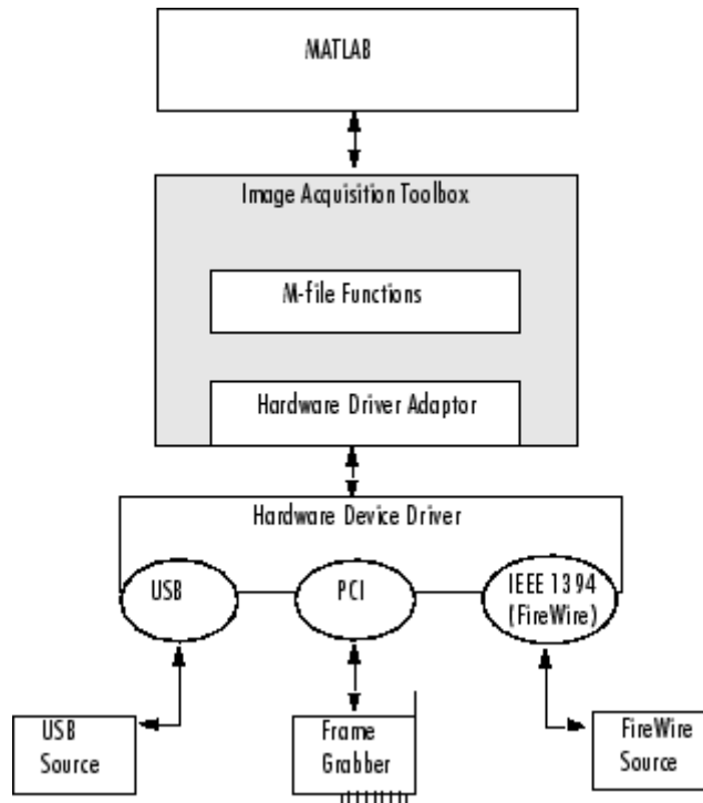
Image Acquisition Toolbox Components
