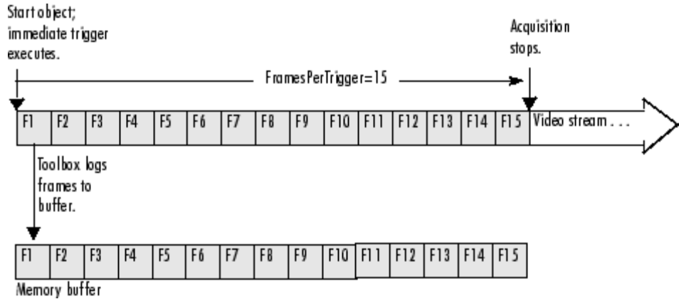
Frames Available After Initial Trigger Execution
